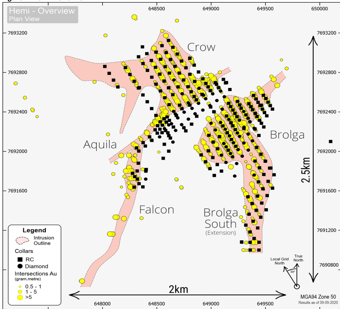
Figure 2: Hemi – Overview
