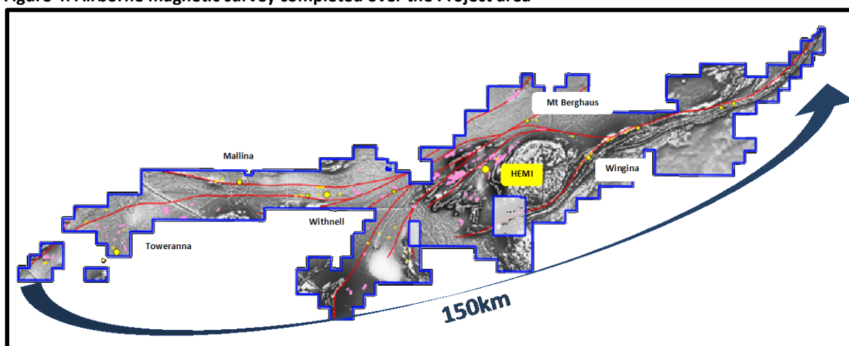
Figure 4: Airborne magnetic survey completed over the Project area
