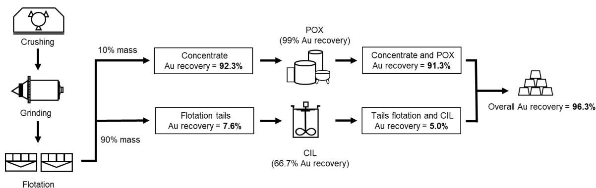
Figure 5: Simplified testwork flowsheet for fresh ore (note: numbers subject to rounding)
